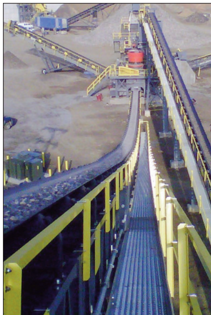
CONVEYOR PARTS
